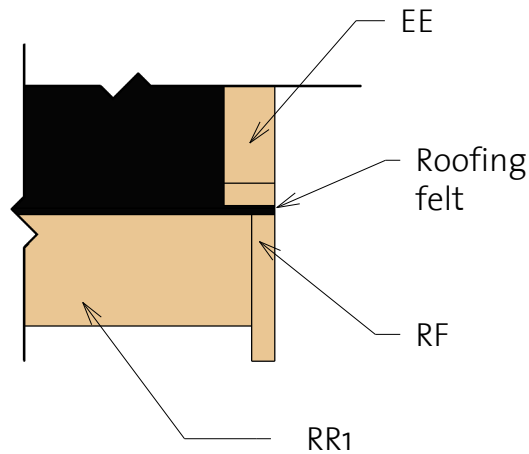
③ Roof Reinforcement
