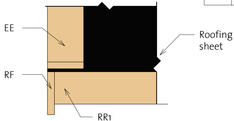
3 Roof Reinforcement
