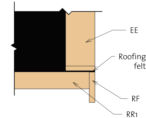
③ Roof Reinforcement
