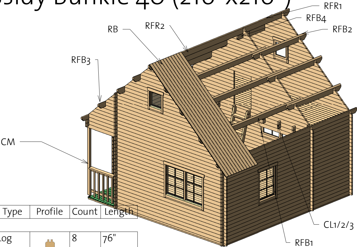
Roof 1
