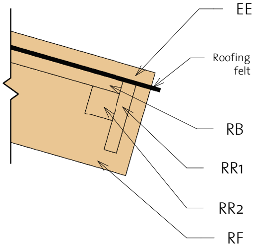
3) Roof Reinforcement
