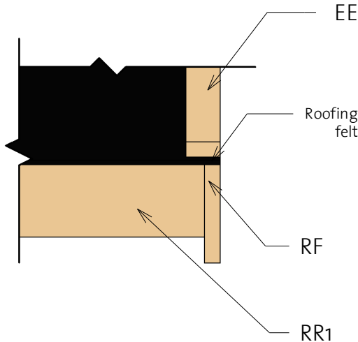
3) Roof Reinforcement
