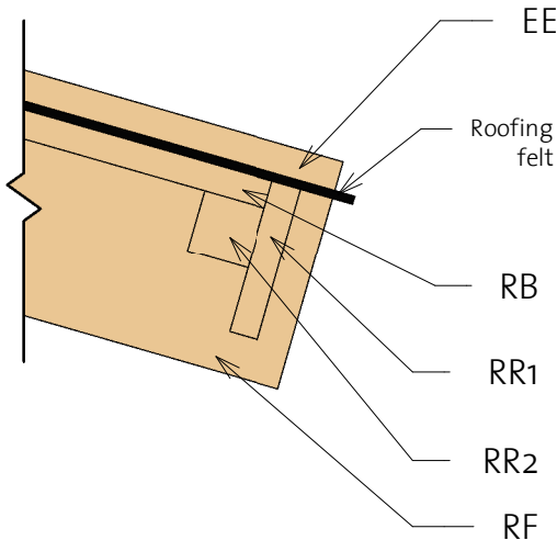
3) Roof Reinforcement
